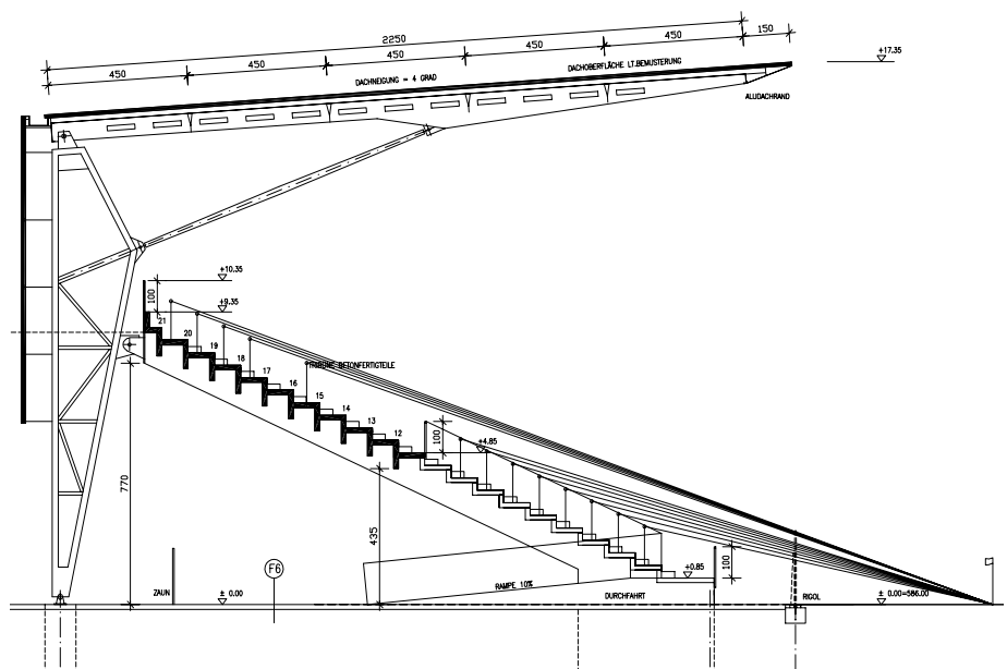
Section North-South: Graphical display of sight lines
